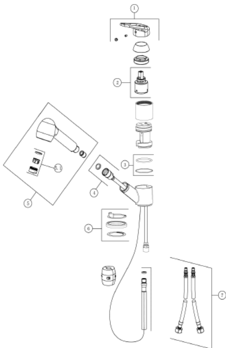
Novara Plus Spray HP Oyster 115.0470.666
