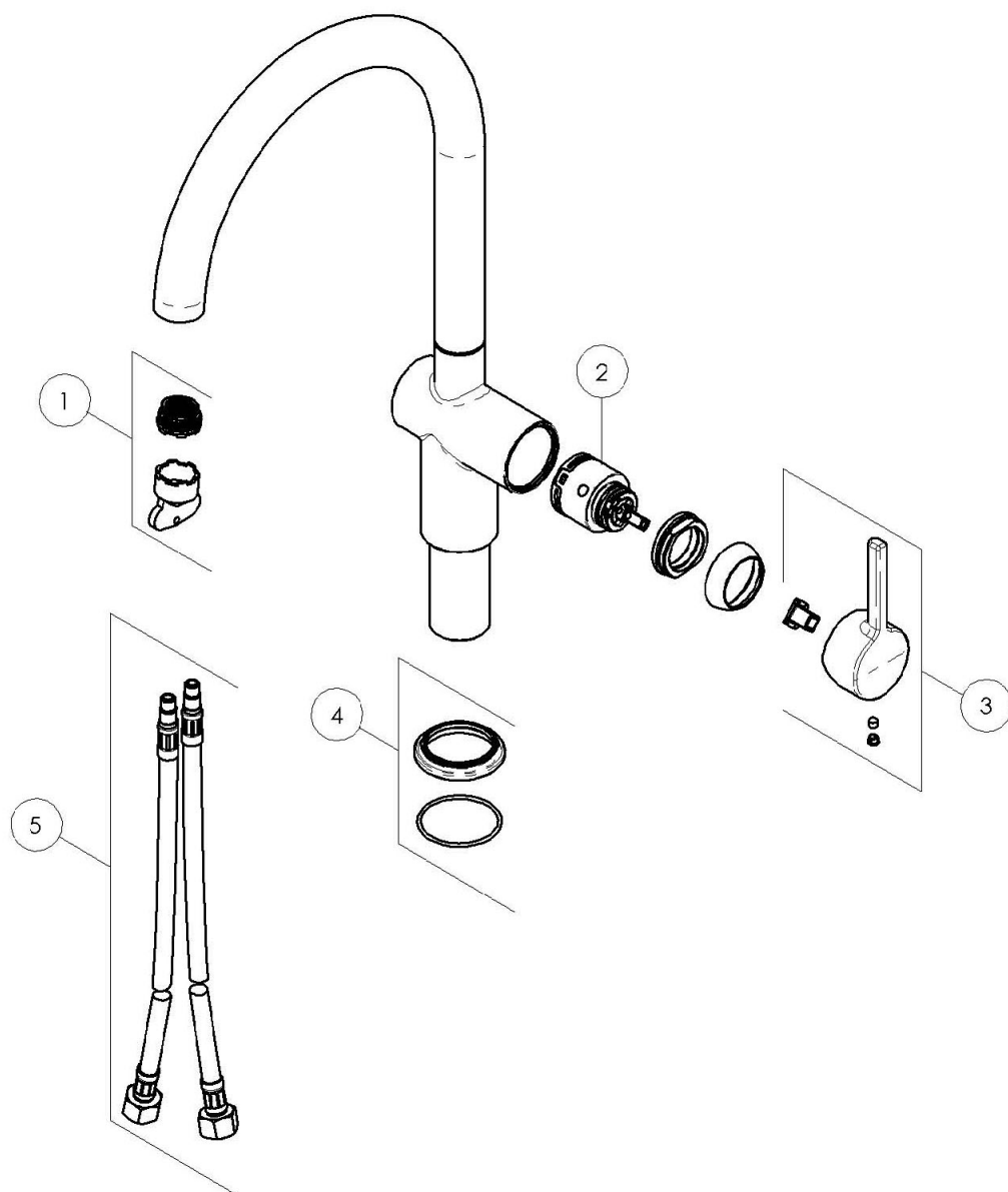
ACTIVE Swivel Spout J 115.0653.396 DS.
