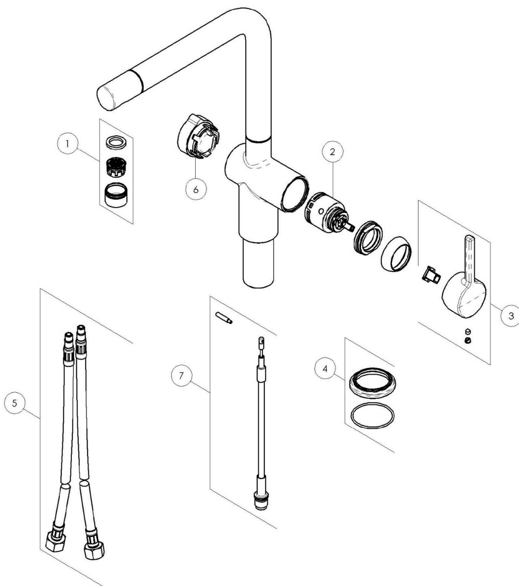
ACTIVE L TWIST swivel 115.0669.768 spout MB
