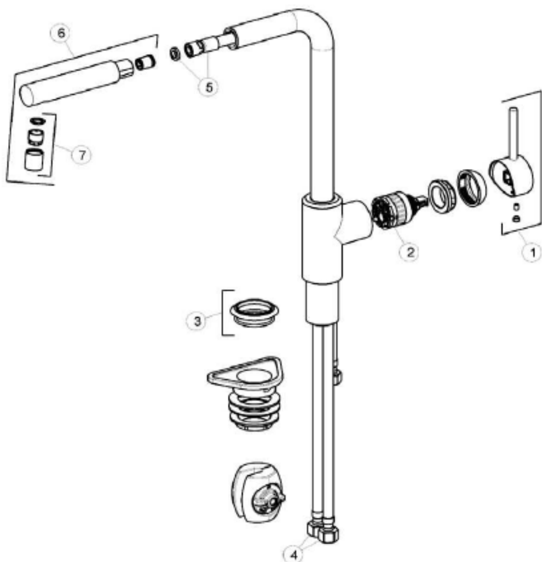
Sirius Side Pull Out Chrome 115.0668.280
