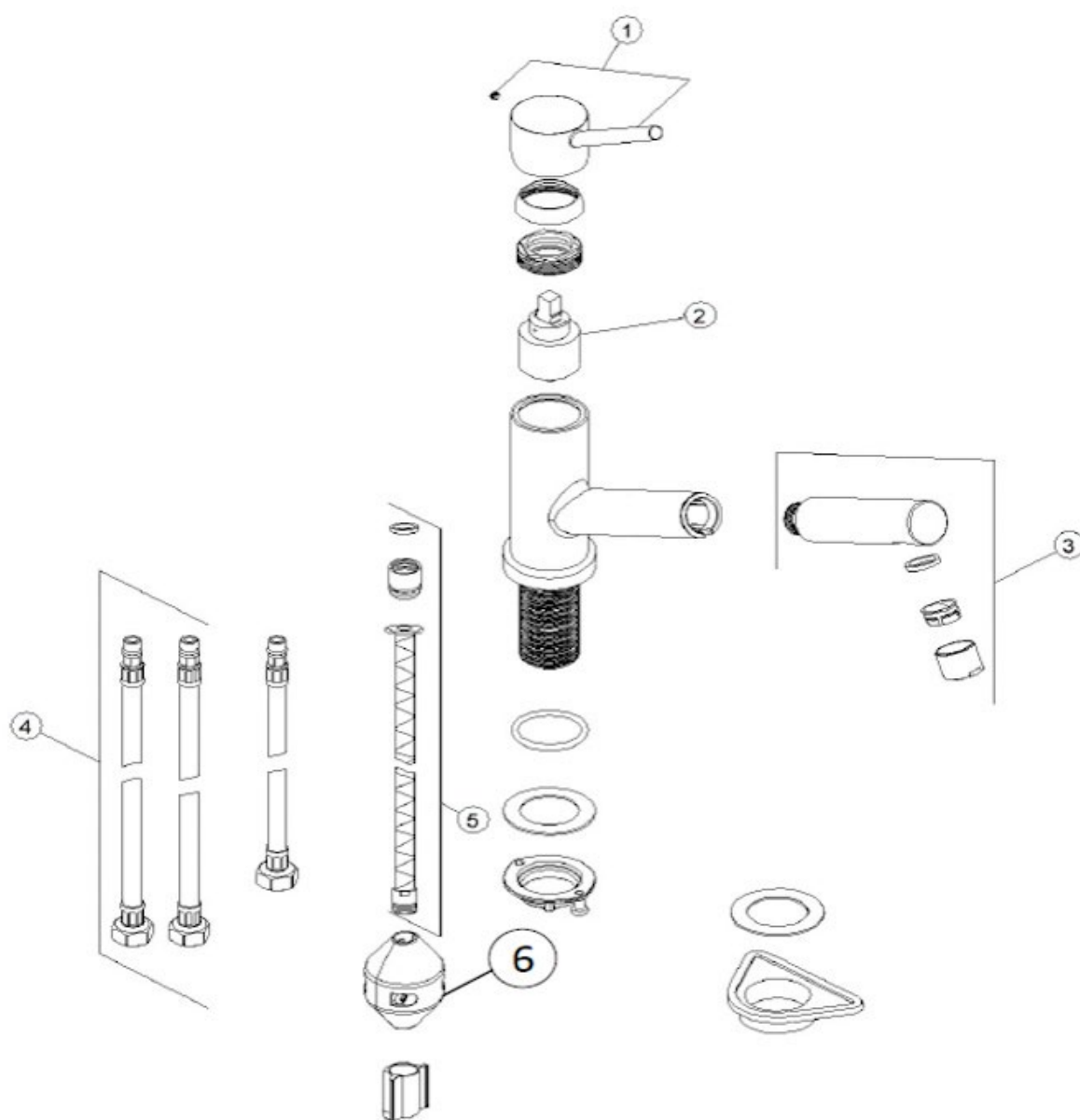
Orbit Pull Out Nozzle Top HP SS 115.0569.461
