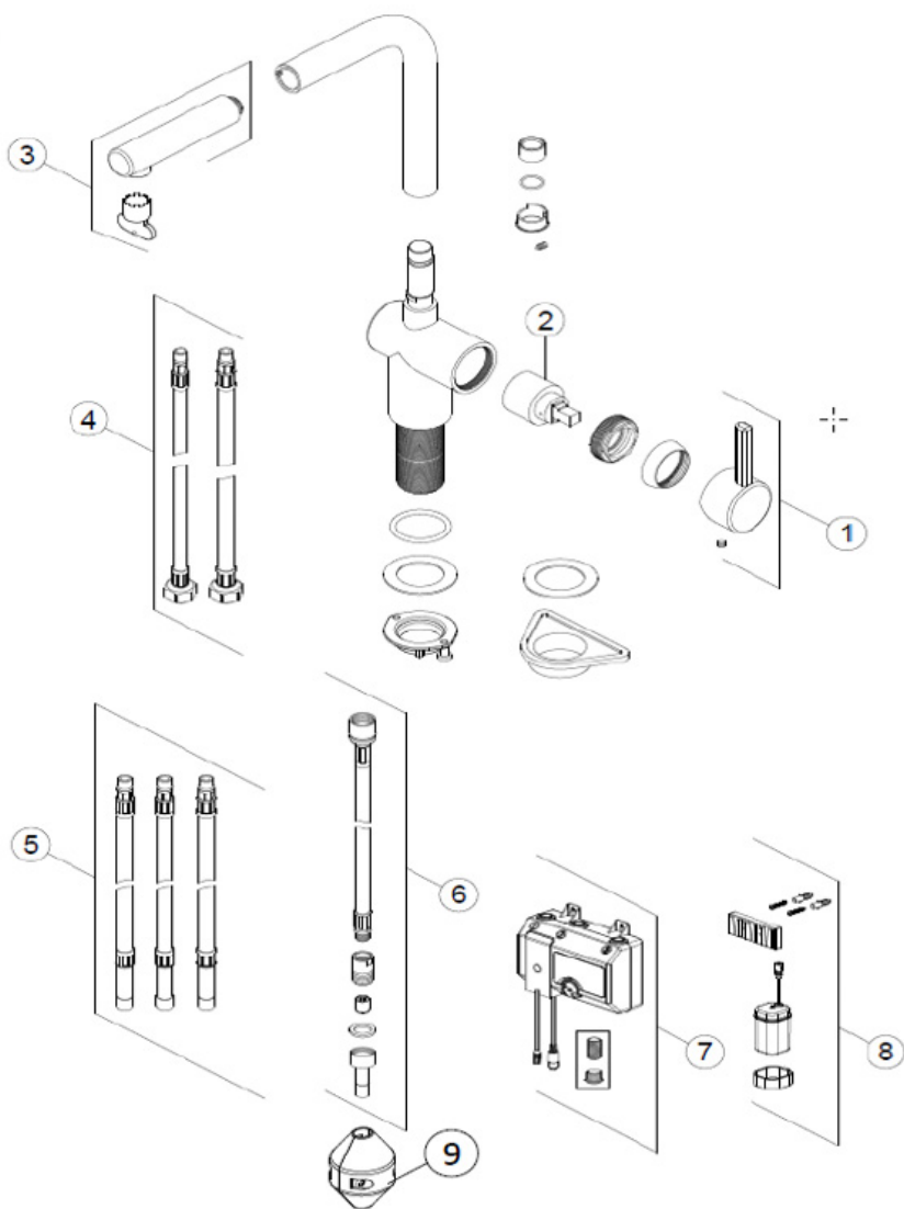
Atlas Neo S Nozzle side HP SS 115.0625.523
