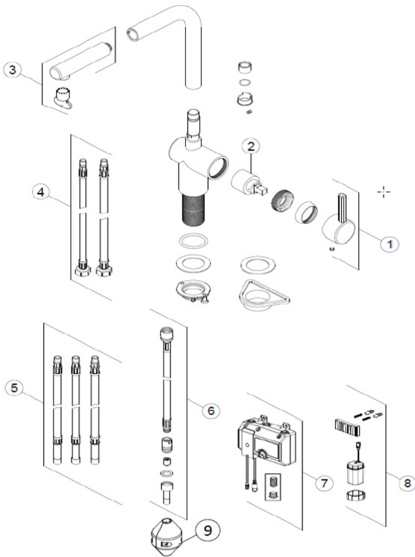
Atlas Neo S Nozzle side HP 115.0625.527 SS IBK
