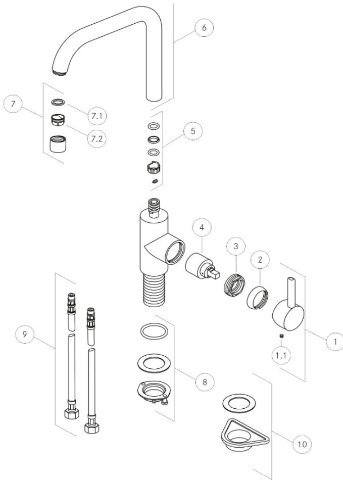
Tap Kubus 330 U spout Side HP SS 115.0529.202
