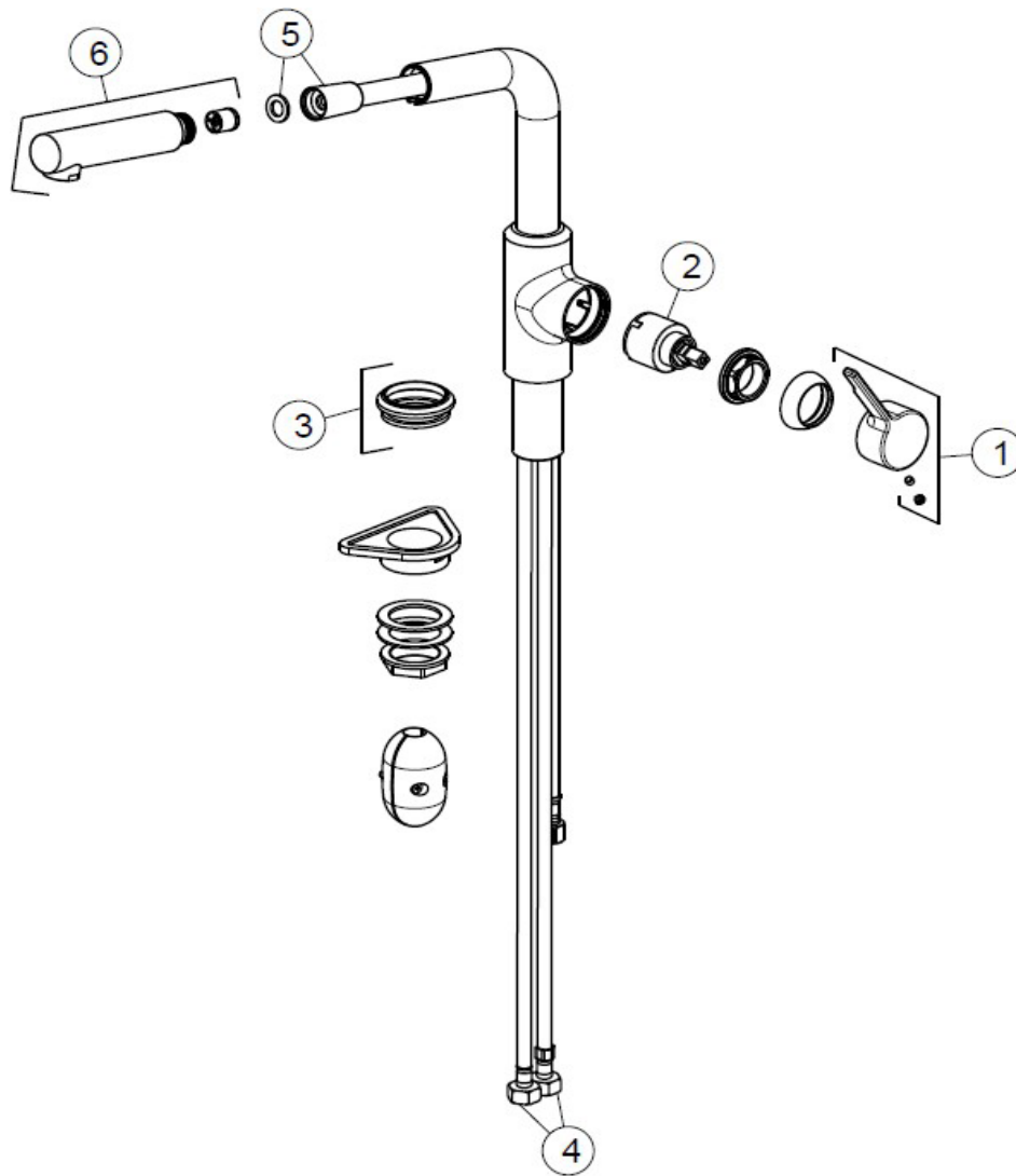
Tap Urban nozzle L-spout side HP ST
