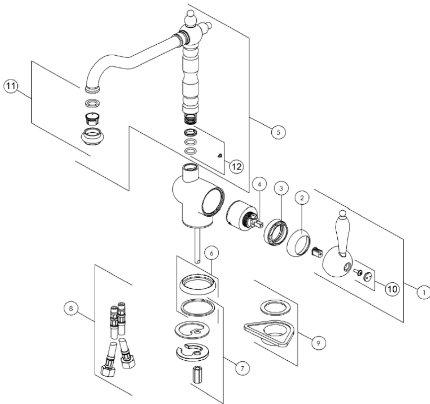
Tap Old England spout side HP CHR 115.0060.360
