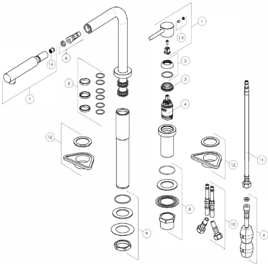
Active Luna nozzle up&down 115.0486.978 HP CHR
