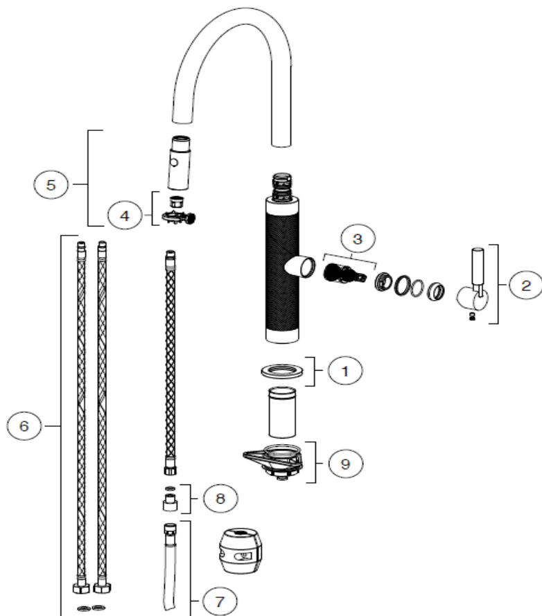
Tap Mythos Masterpiece J PullDown Spray HP SS
