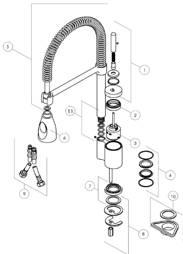
Tap Joy Cocktail PRO side HP CHR 115.0029.591
