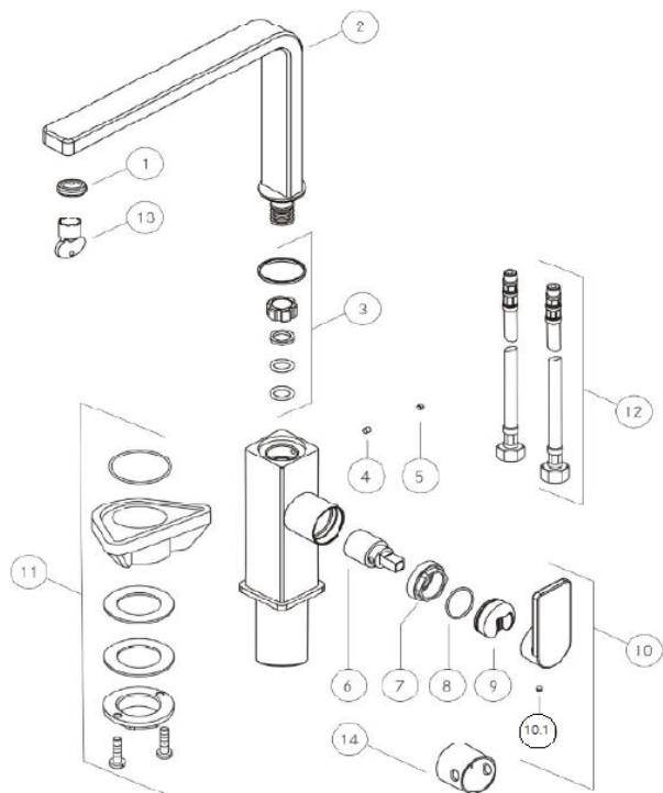
Tap Mythos Swivel Side HP Industr 115.0550.441 Black
