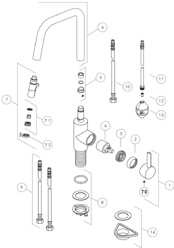
Tap Kubus 330 U spout Side HP SS 115.0529.202
