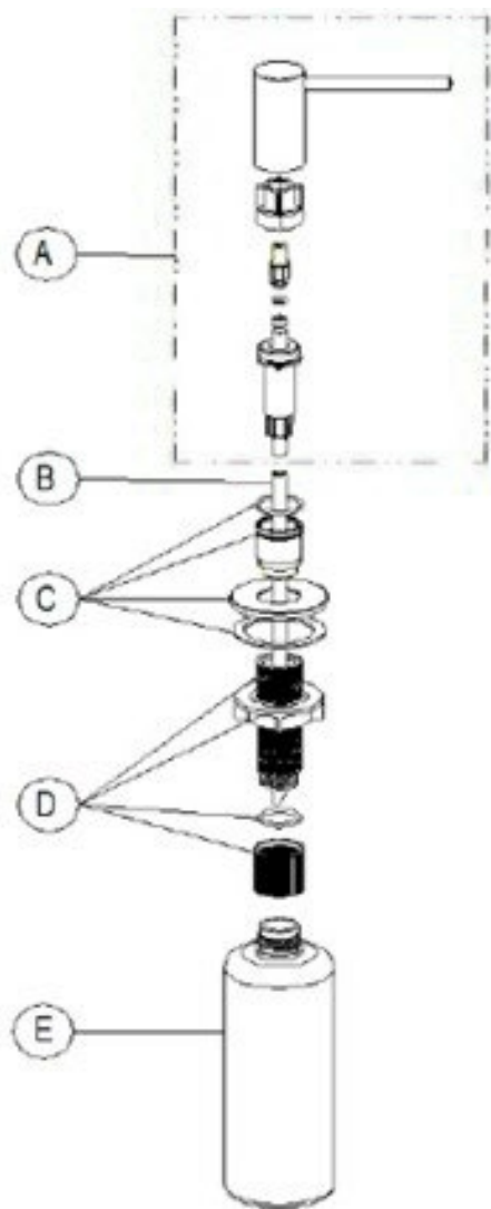
SD Atlas Stainless Steel Anthracite 112.0717.103
