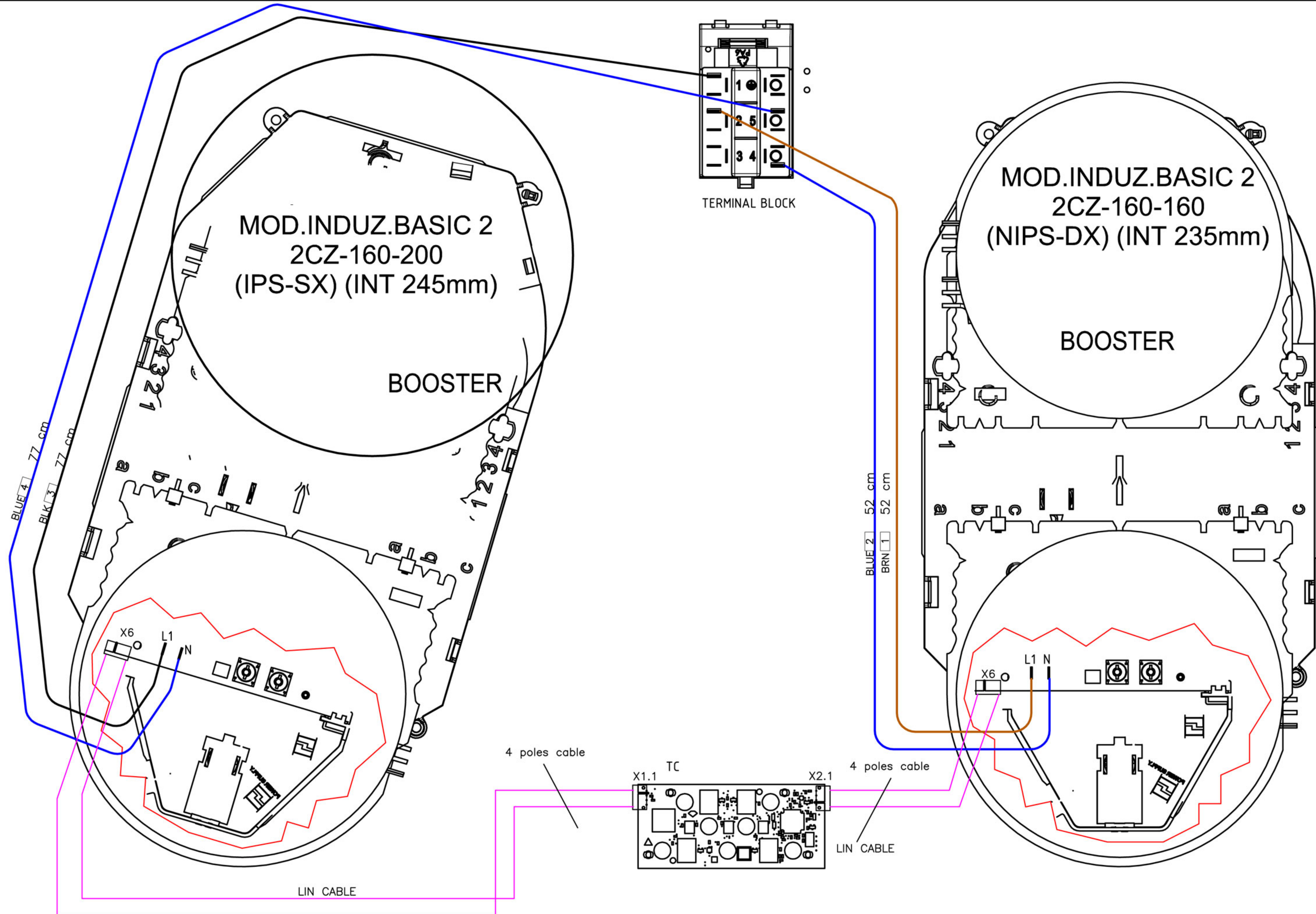
SUPPLY CABLE CONNECTION OPTIONS SUPPLY CORD 4X2.5mmq H05V2V2-F
