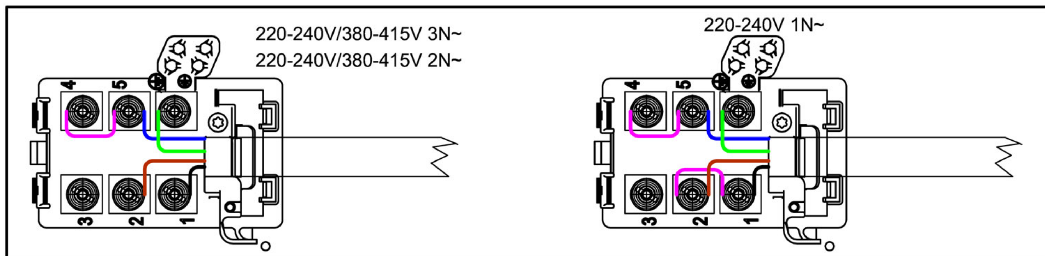
SUPPLY CABLE CONNECTION OPTIONS SUPPLY CORD 4X2.5mmq H05V2V2-F
