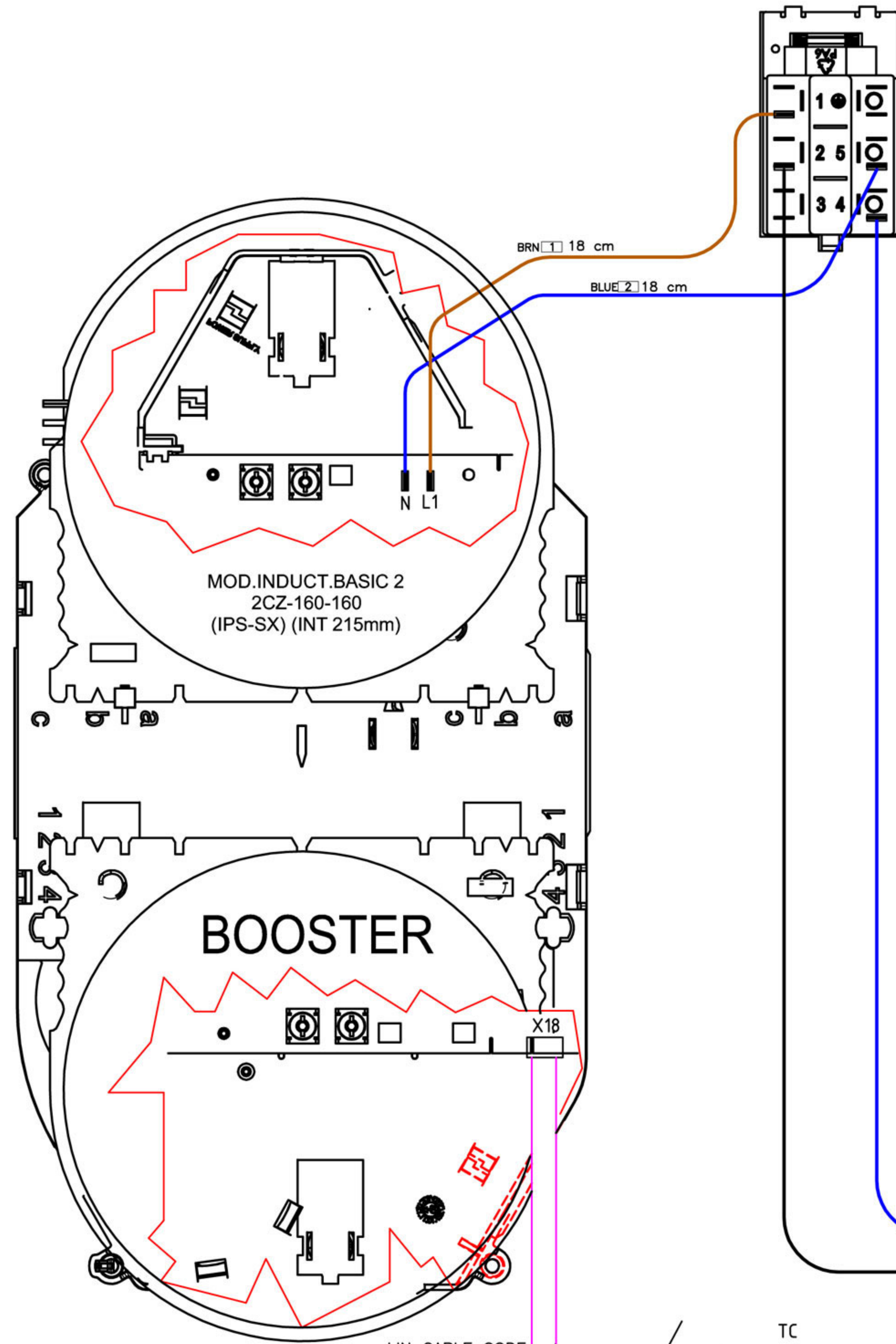
SUPPLY CABLE CONNECTION OPTIONS SUPPLY CORD 4X2.5mmq H05V2V2-F
